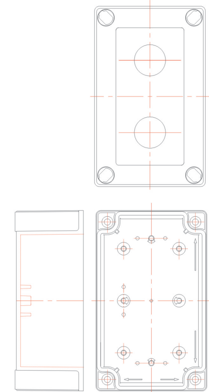
Tailor drilled push button holes (Article No. 011 70 0229)
