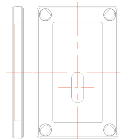
Tailor made cutout (Article No. 01 17 00101)
